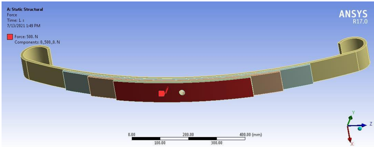
FIG 4.3 LOADING
