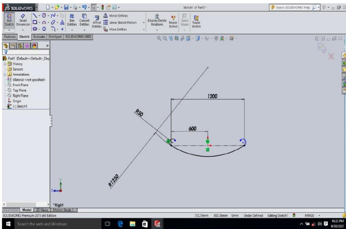
FIG 5.1 SKETCH OF MASTER LEAF
