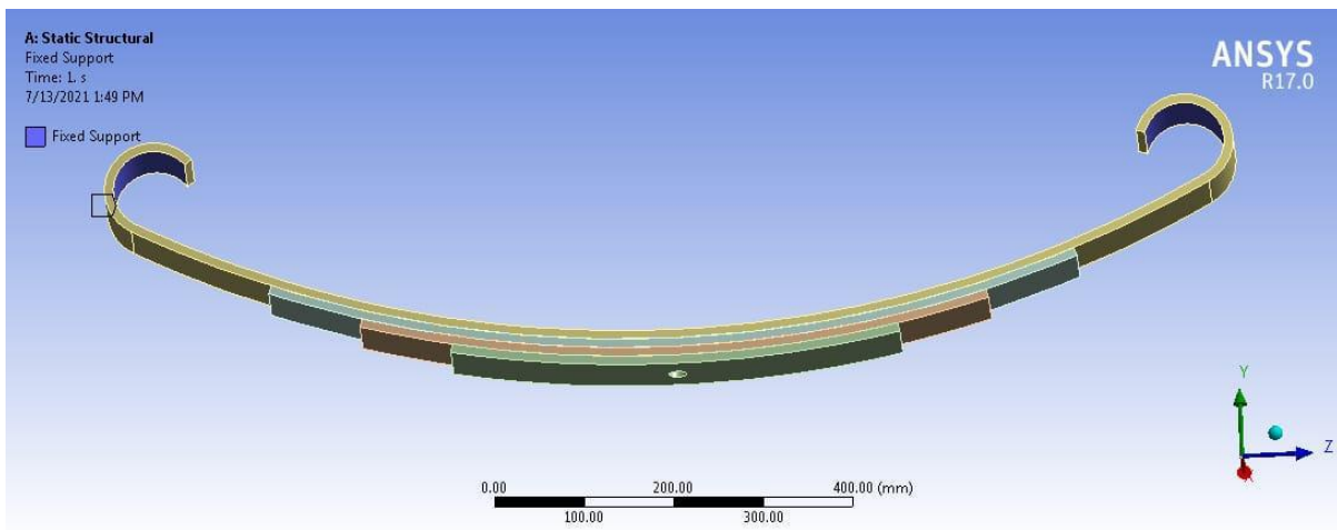
FIG 4.2 FIXED SUPPORTS
