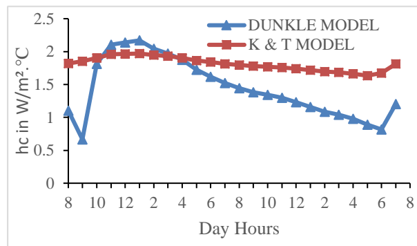
Figure 4 c : Variation of h_{cw} for 2kg sizes of paraffin wax
