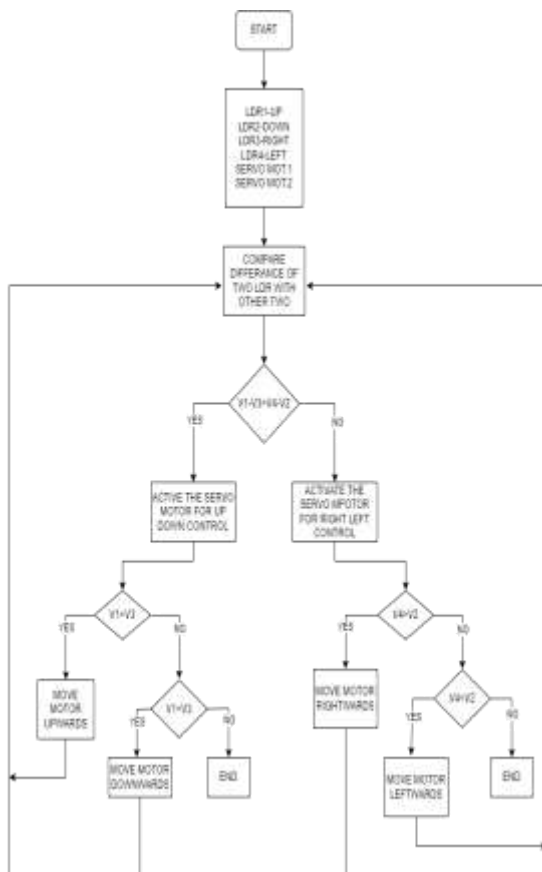
FIG : Flow chart of solar tracking system
