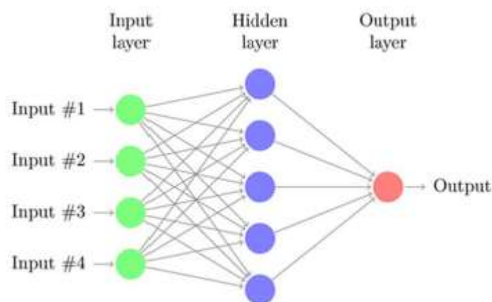
Figure 1: Neural Network.
