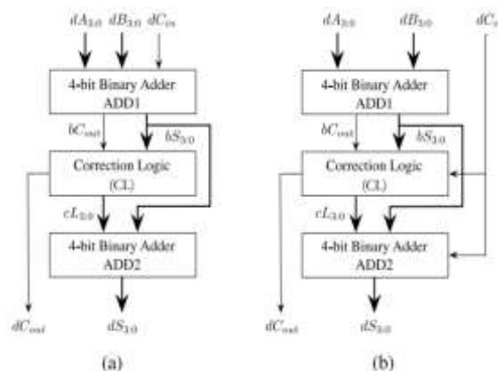
Fig. 2. BCD adder block diagrams (a) conventional design and (b) suggested design.
