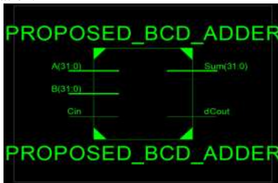
Fig4: RTL Schematic of Proposed BCD adder
