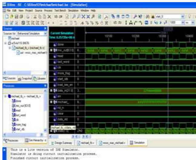
Figure 6 Simulation Waveform of Hardware and software of TKIP Michel block
