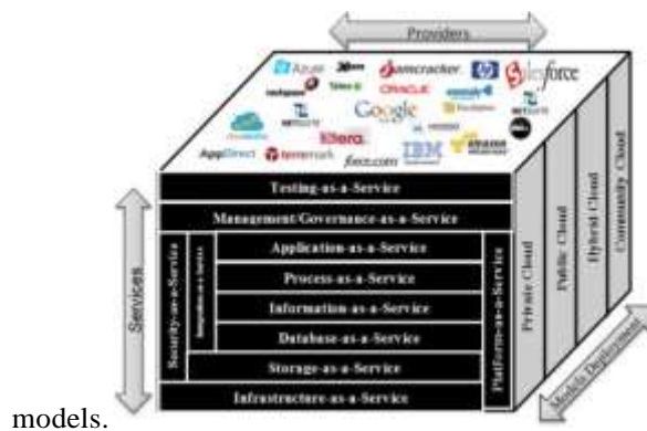
Figure 1. The Relationship between Services, Deployment Models, and Providers
