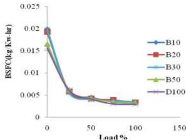
Figure 3 Variation of (BSFC) with Loads for Waste Coconut Oil Biodiesel Blends with Diesel
