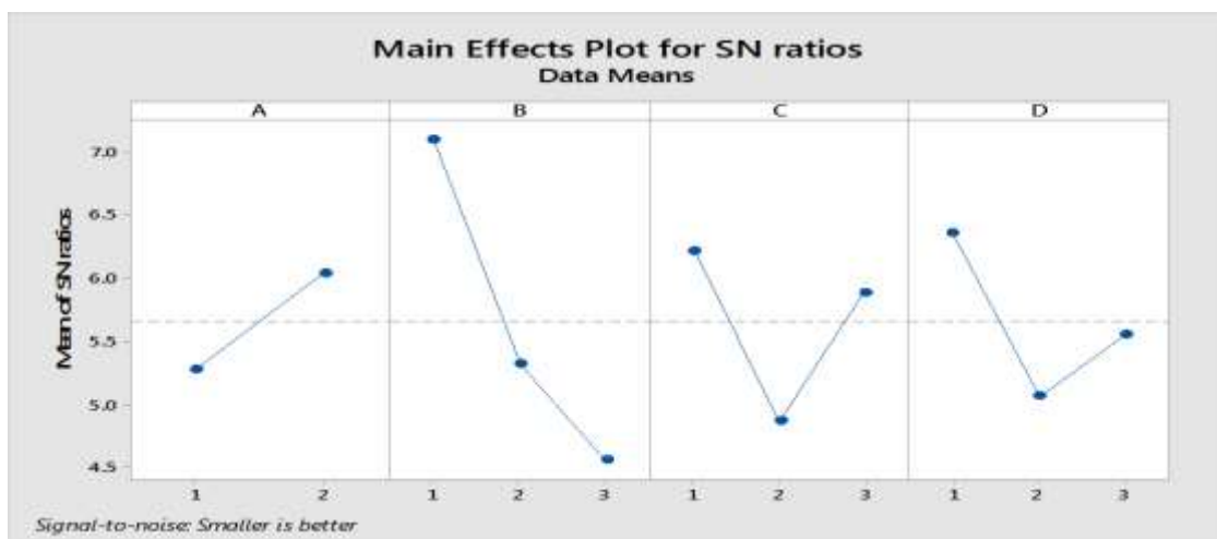
Figure 2. Main Effect plot for Surface Roughness
