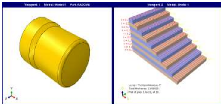
Figure 2 Layup Configuration (2mm)
