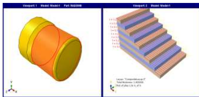
Figure 6 Layup Configuration (1.8mm)
