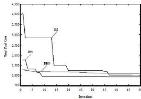
Fig. 6 Convergence Characteristics Between IHS, HS, BBO with Valve point loading
