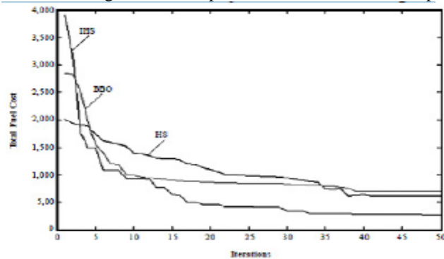
Fig. 4 Convergent characteristic of all algorithms
