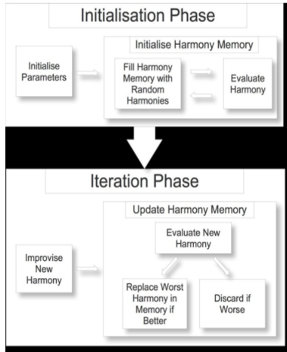
Fig. 3: Block Diagram of Harmony search Algorithm
