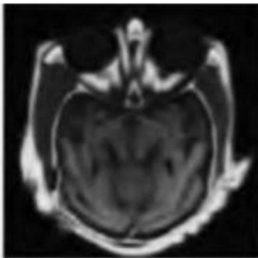
Figure 5.Wavelet transform method
