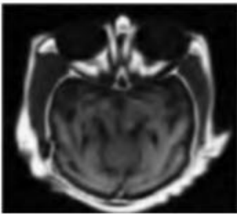
Figure 4.Pixel value maximization.
