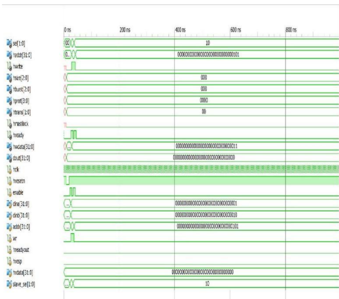
Figure: Master operation
