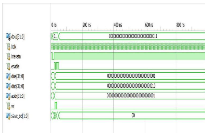
Figure: One Master and Slave operation
