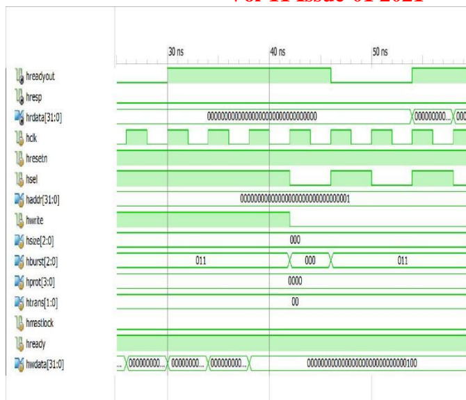
Figure: Slave operation
