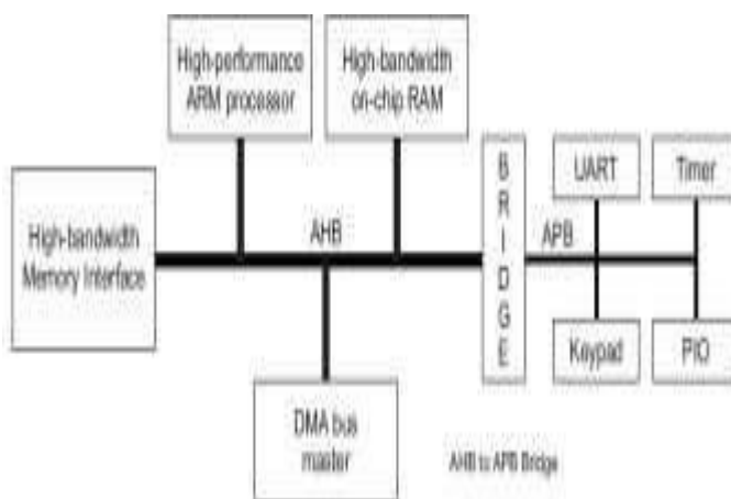
Figure 1 AMBA based system
