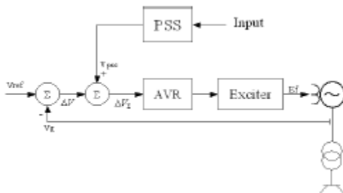
Fig.3.2: block diagram of supplementary control loop for the AVR system.
