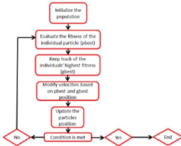
Fig 4.1: PSO Algorithm Chart
