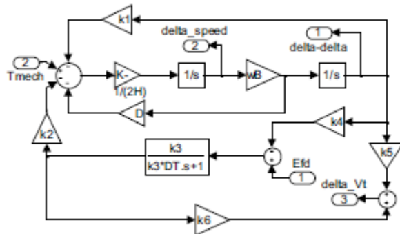
Fig.5.2: overall representation of synchronous machine
